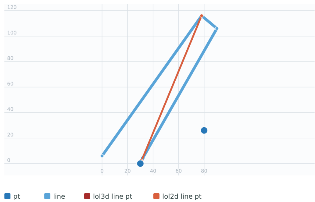
Longest line between a Polygon and a MultiLineString, comparing the 3D and 2D results.
