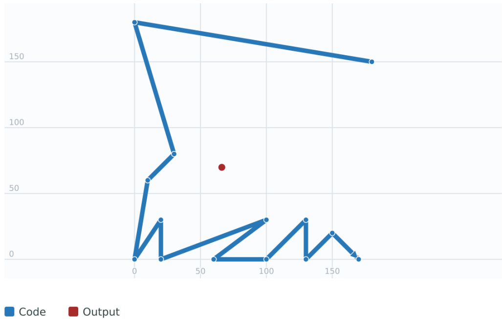
Centroid of a Polygon.
