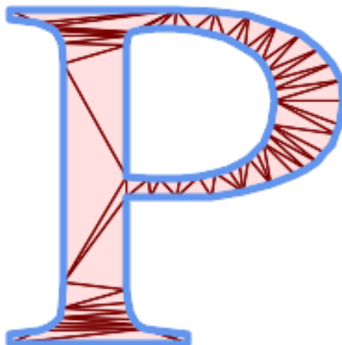
Polygontriangulering
