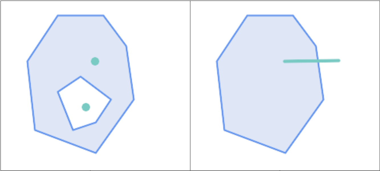
POLYGON/MULTIPOINT
