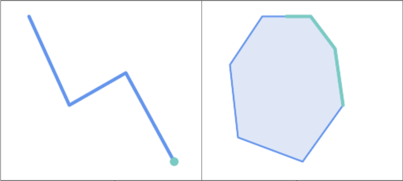
LINESTRING/POINT
