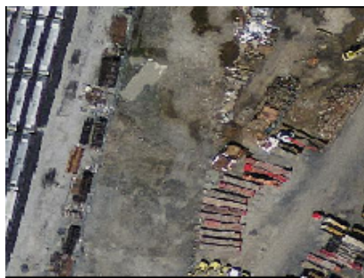
After transform to wgs 84 long lat (wgs_84)
